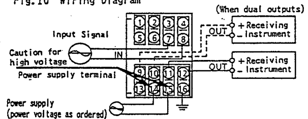
Fig.10 Wiring Diagram
